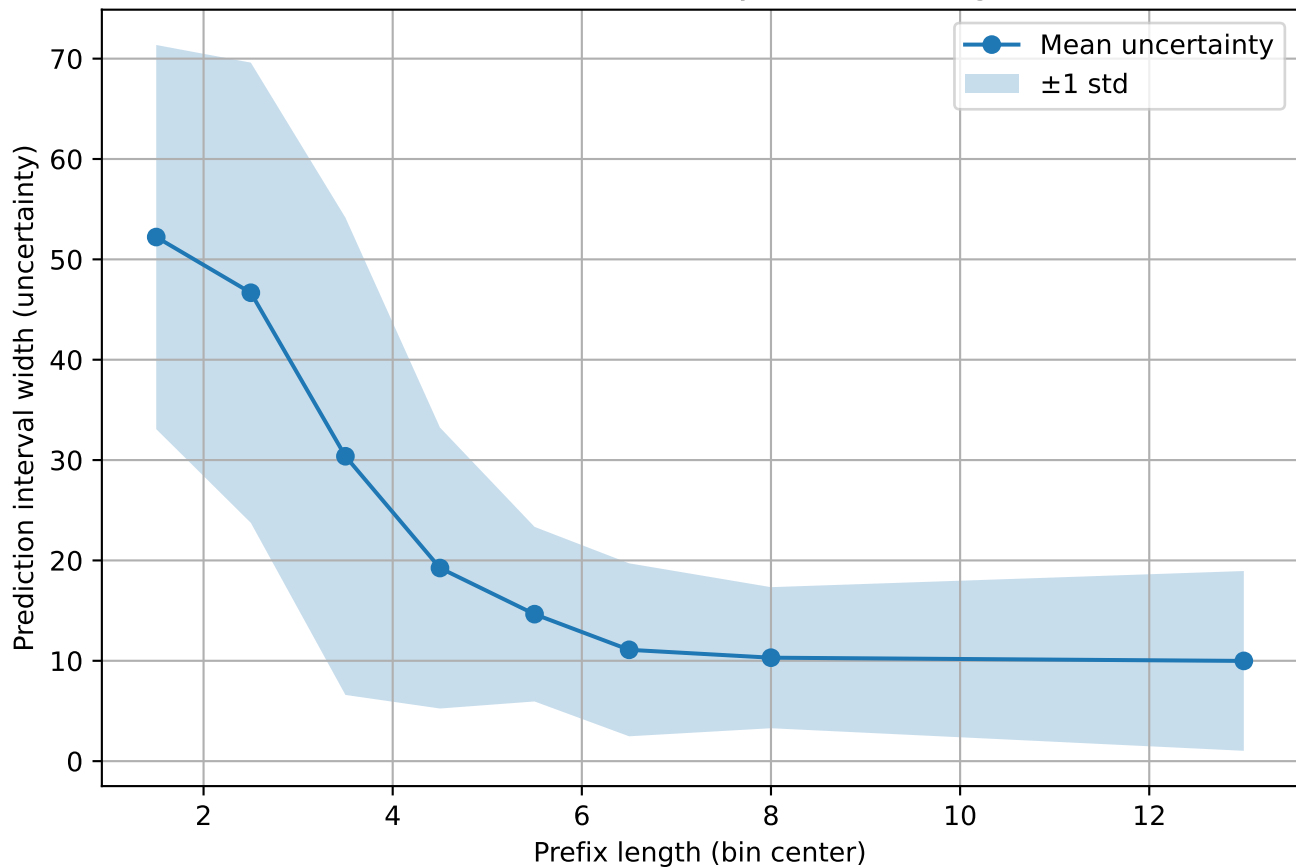
BPIC20PTC: Uncertainty vs Prefix Length
